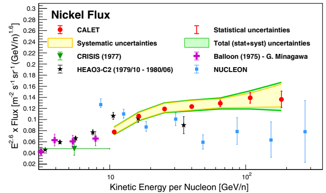
FIG. 2. CALET nickel flux (multiplied by E^{2.6} ) as a function of kinetic energy per nucleon. Error bars of the CALET data (red) represent the statistical uncertainty only, the yellow band indicates the quadrature sum of systematic errors, while the green band indicates the quadrature sum of statistical and systematic errors. Also plotted are the measurements from Balloon 1975 [32], CRISIS [34], HEAO3-C2 [27], and NUCLEON [28]. This figure is reproduced and enlarged in Fig. S9 of the Supplemental Material [53].
