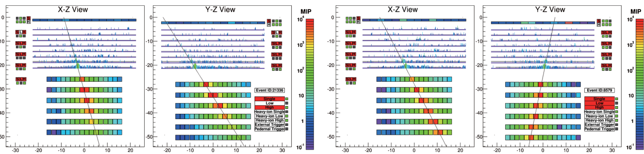
FIG. 1. Examples of TeV event candidates showing energy deposit in each detector channel in the X-Z and Y-Z views. (Left) An electron (or positron) candidate (reconstructed energy of 3.05 TeV and energy deposit sum of 2.89 TeV). (Right) A proton candidate (energy deposit sum of 2.89 TeV).
