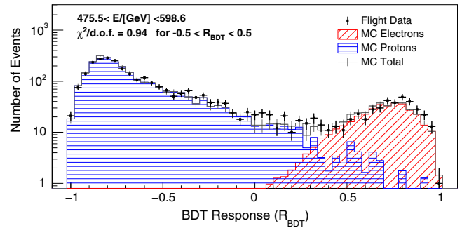
FIG. 2. An example of BDT response distributions in the 476 < E < 599 GeV bin including all acceptance conditions A , B , C , and D . The BDT response distributions for the TeV region are shown in Fig. 2 of the Supplemental Material [16].
