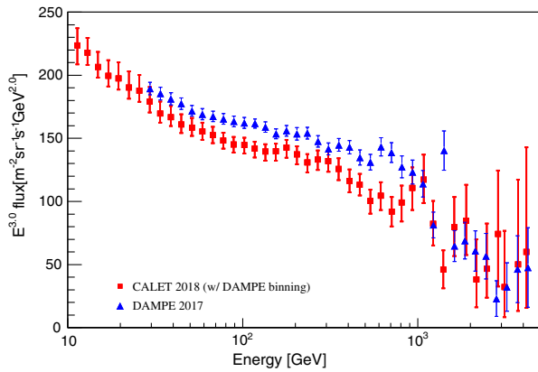
FIG. 4. Cosmic-ray all-electron spectrum measured by CALET from 10.6 GeV to 4.57 TeV using the same energy binning as DAMPE’s result [7] and compared with it. The error bars indicate the quadratic sum of statistical and systematic errors (not including the uncertainty on the energy scale).
