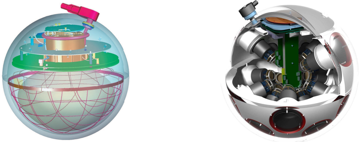
Figure 35.5: Schematic views of the digital OMs of IceCube (left) and KM3NeT (right).
