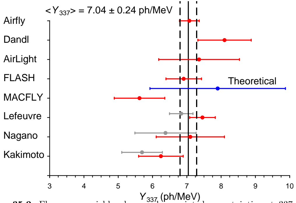
Figure 35.2: Fluorescence yield values and associated uncertainties at 337 nm ( Y_{337} ) in dry air at 800 hPa and 293 K (Figure from [12]). The methodology and corrections that were applied to obtain the average and the uncertainty are discussed extensively in this reference. The vertical axis denotes different laboratory experiments that measured FY. The gray bars show three of the original measurements to illustrate the scale of the corrections applied.
